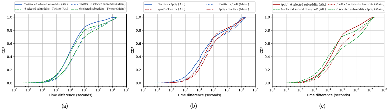
Figure 7: CDF of the difference between the first occurrence of a URL between (a) six selected subreddits and Twitter, (b) /pol/ and Twitter, and (c) /pol/ and six selected subreddits.
