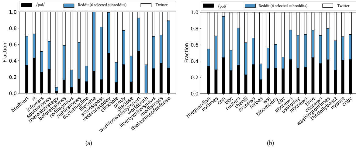
Figure 2: Top 20 domains and each platform’s fraction for (a) alternative and (b) mainstream news.
